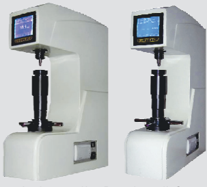
Automatic Rockwell & Automatic Rockwell Superficial Hardness Tester
